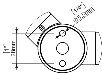
WALL FIXATION / ANCLAJE PARED
