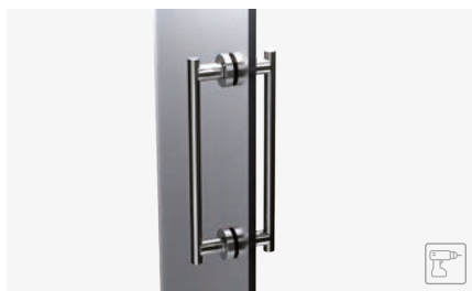
SHOWER DOOR HANDLE IN & OUT 500MM. ASA 500 MM. DOBLE MAMPARA CHROME Ref. 152957 € 94,00 A: 510 mm. B:50 C: 139 mm. D: 460 mm.
